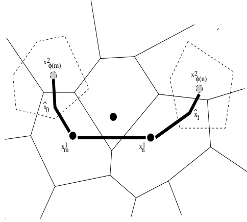
FIG. 4. Path constructed in Theorem 4.5.
