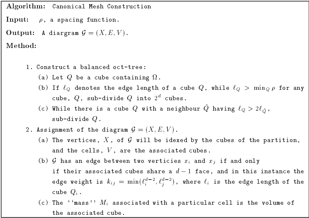
FIG. 5. Constructing the canonical mesh.
