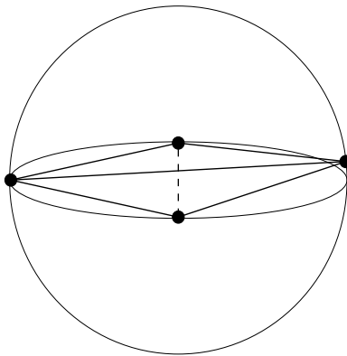
FIG. 1. Sliver and circum sphere.
