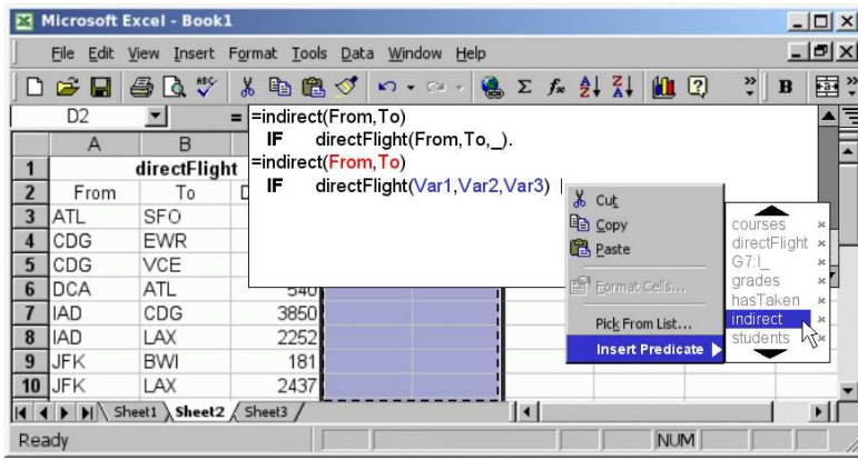
Figure 1: Mouse-Assisted Clausal Definition
