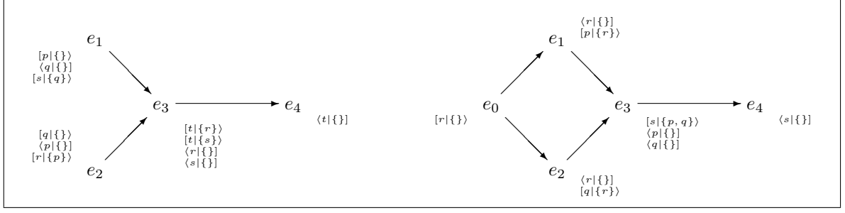
Figure 1. Reasoning with Extensions versus Reasoning with Completions
