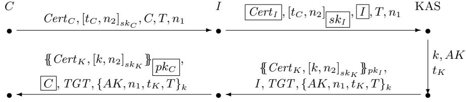
Fig. 2. Message Flow in the Man-In-The-Middle Attack on PKINIT-26, where TGT = \{AK, I, t_K\}_{k_T} .
