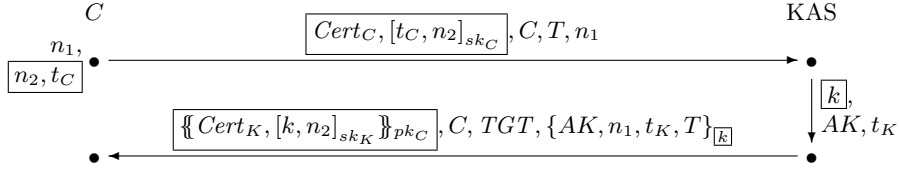
Fig. 1. Message Flow in the Traditional AS Exchange and in PKINIT-26 , where TGT = \{AK, C, t_K\}_{k_T} .
