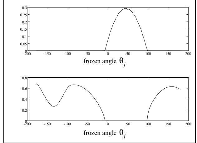
Figure 6: The penalty function and the measure of isotropy.
