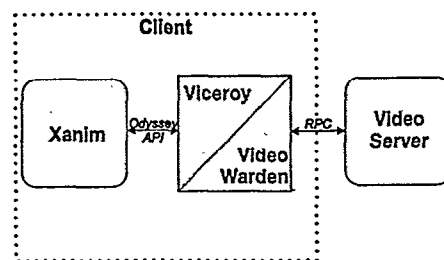
Figure 4: Video Player in Odyssey
